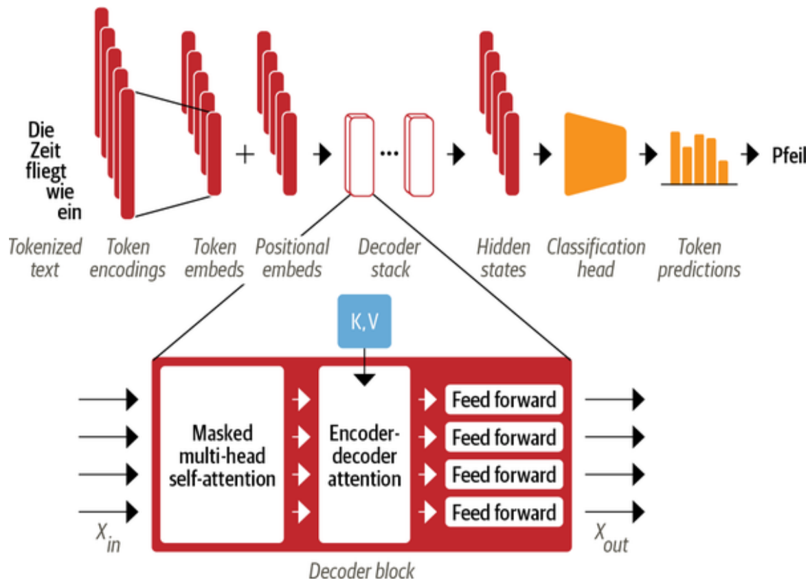
Figure 3-7. Zooming into the transformer decoder layer
