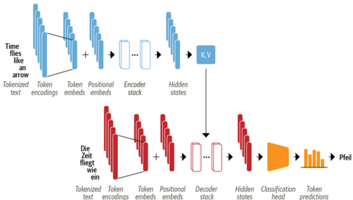
Figure 3-1. Encoder-decoder architecture of the transformer, with the encoder shown in the upper half of the figure and the decoder in the lower half
