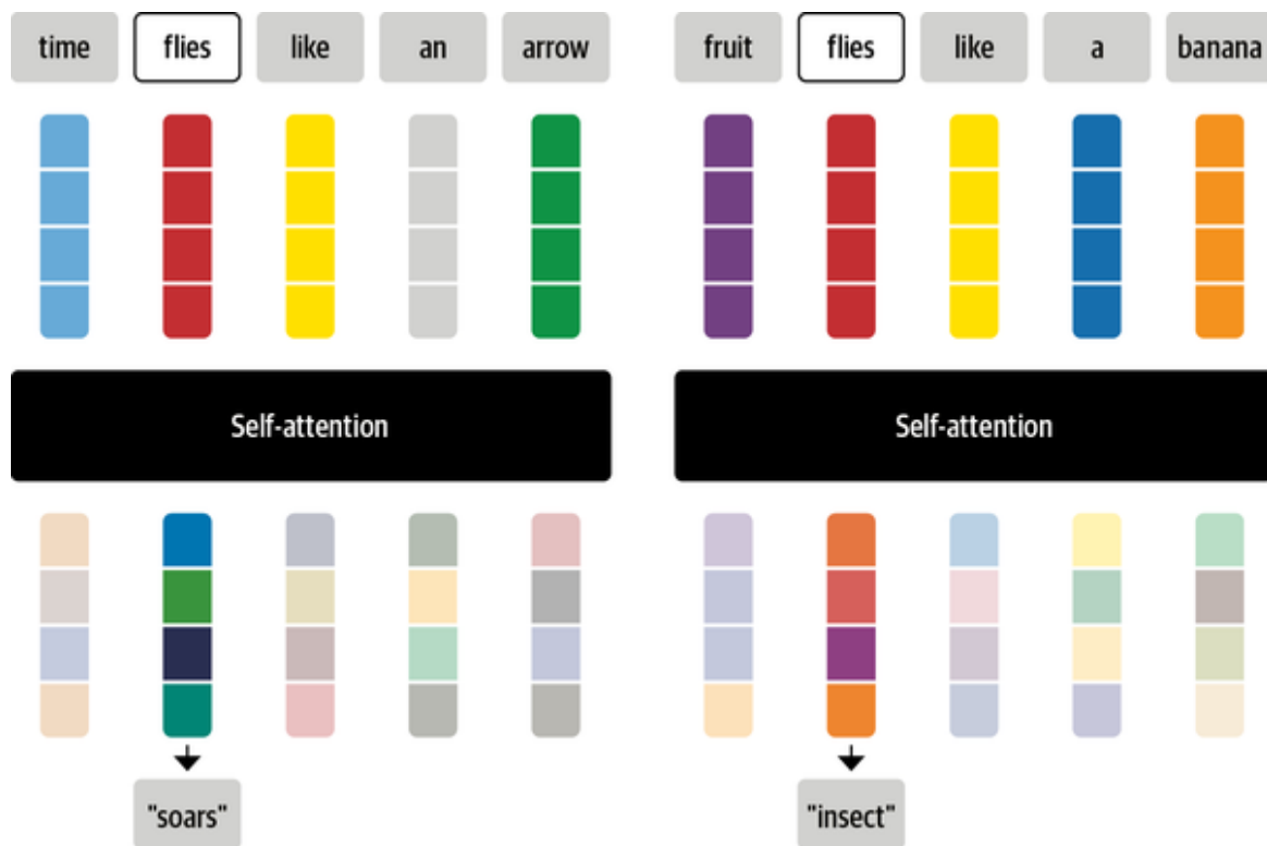
Figure 3-3. Diagram showing how self-attention updates raw token embeddings (upper) into contextualized embeddings (lower) to create representations that incorporate information from the whole sequence
