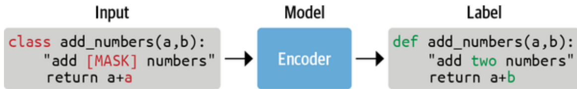
Figure 10-3. In masked language modeling some of the input tokens are either masked or replaced, and the model's task is to predict the original tokens; this is the architecture underlying the encoder branch of transformer models
