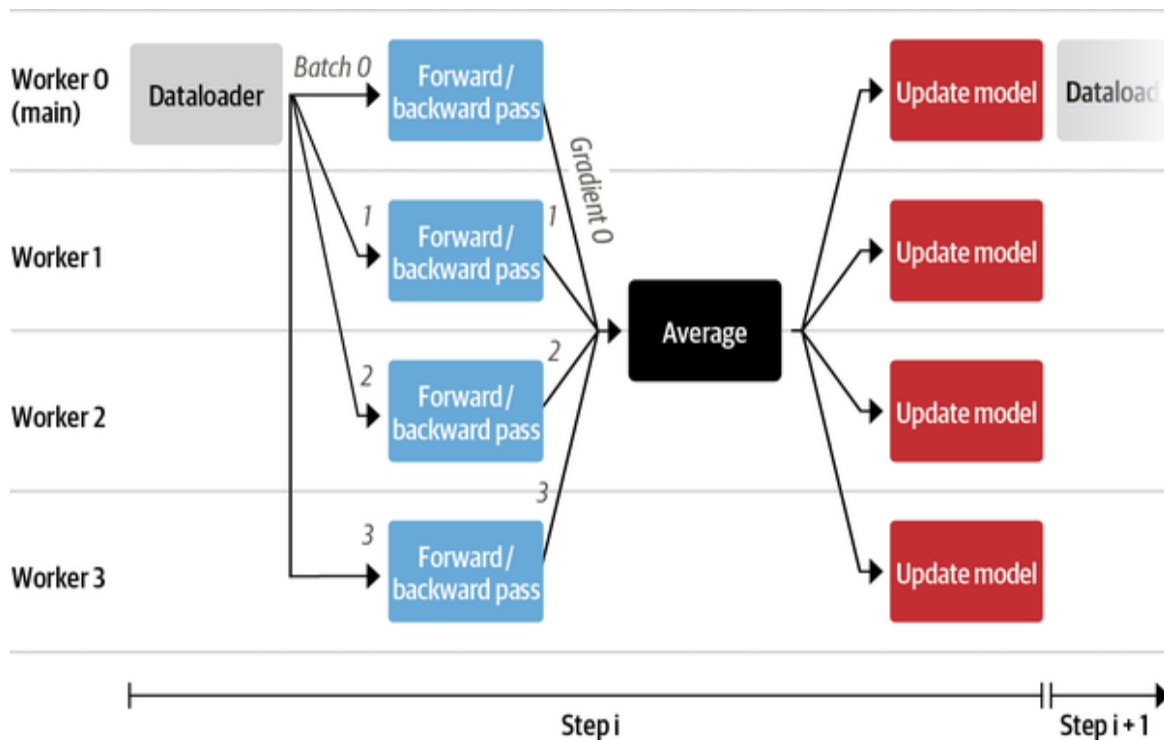
Figure 10-6. Illustration of the processing steps in DDP with four GPUs
