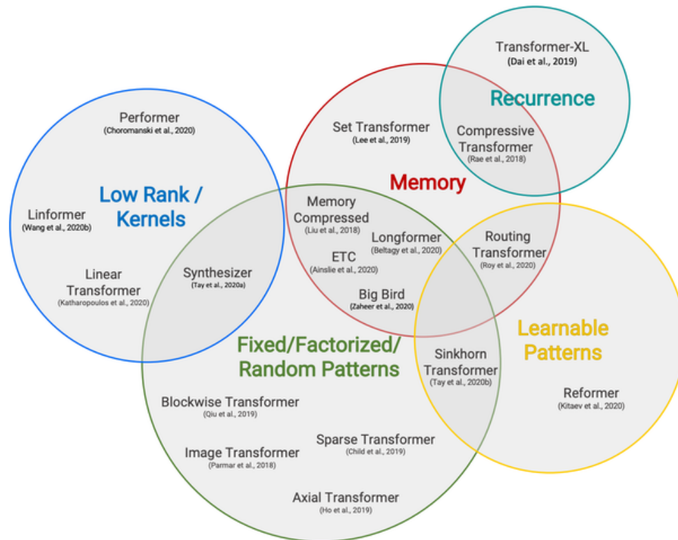
Figure 11-4. A summarization of research directions to make attention more efficient (courtesy of Yi Tay et al.) 6
