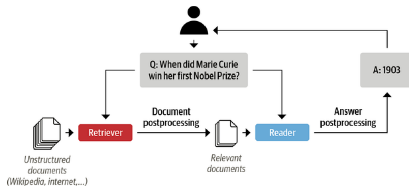
Figure 7-9. The retriever-reader architecture for modern QA systems
