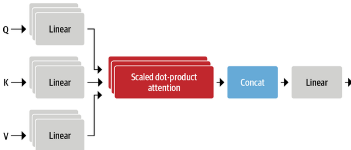
Figure 3-5. Multi-head attention
