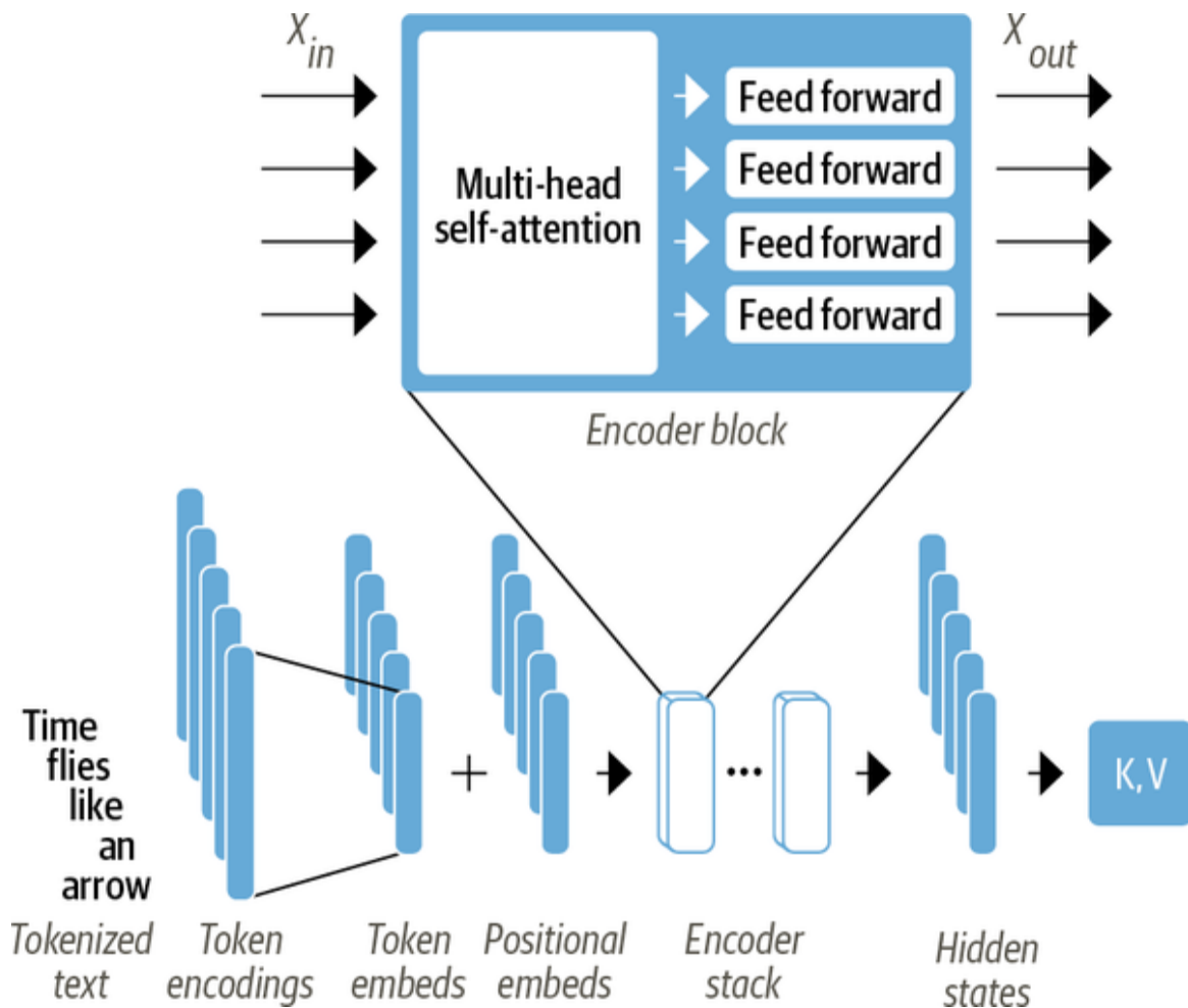
Figure 3-2. Zooming into the encoder layer
