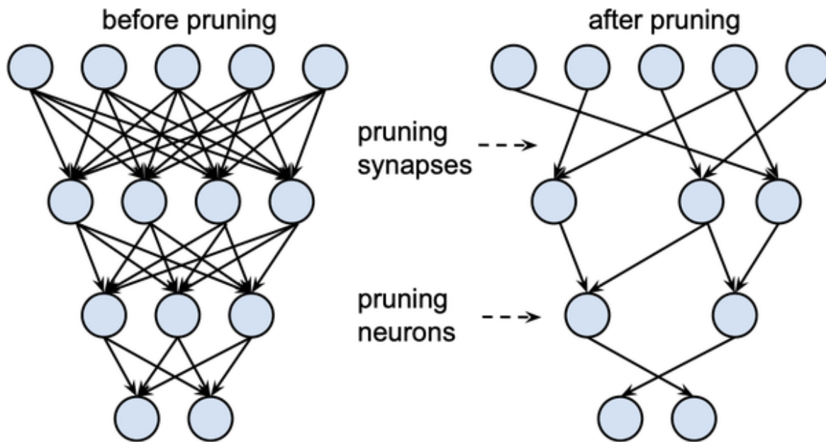
Figure 8-10. Weights and neurons before and after pruning (courtesy of Song Han)
